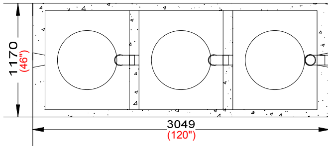
Top Section
