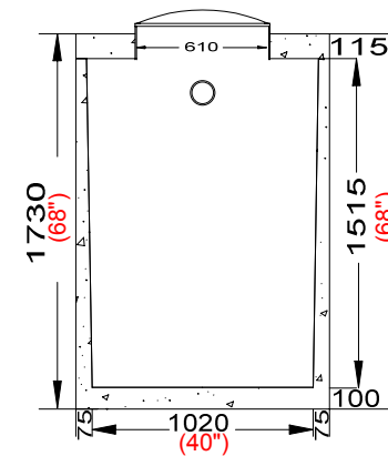
End Section
