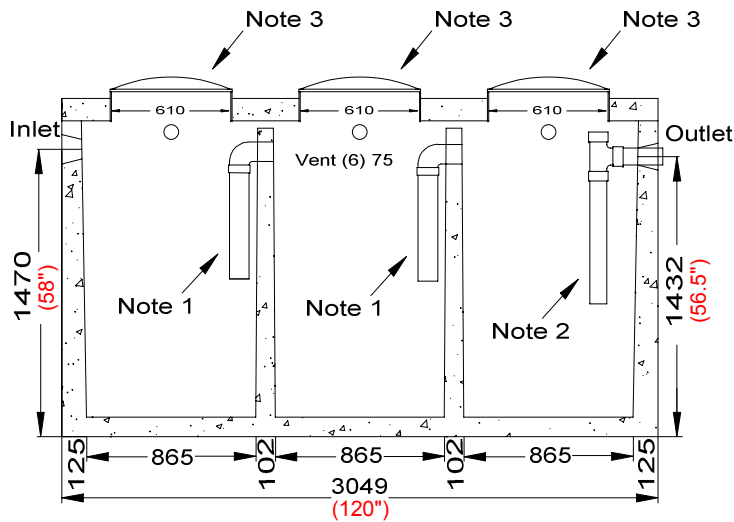
Side Section
