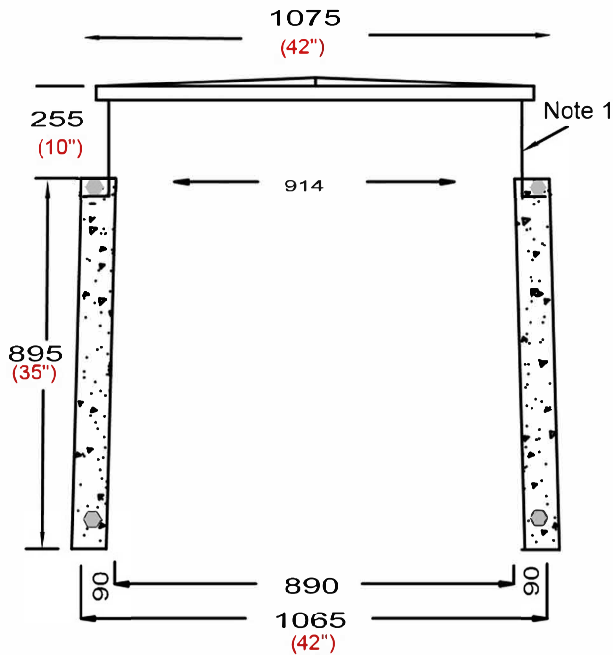
End Elevation Section
