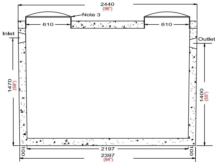
Side Elevation Section
