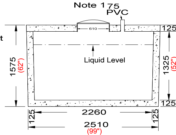
End Elevation Section
