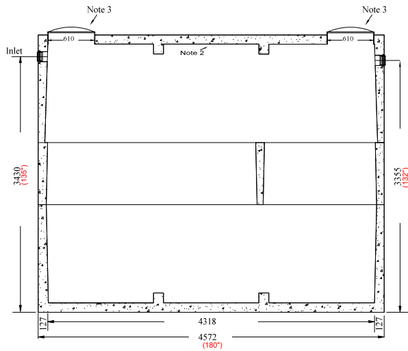
Side Elevation Section
