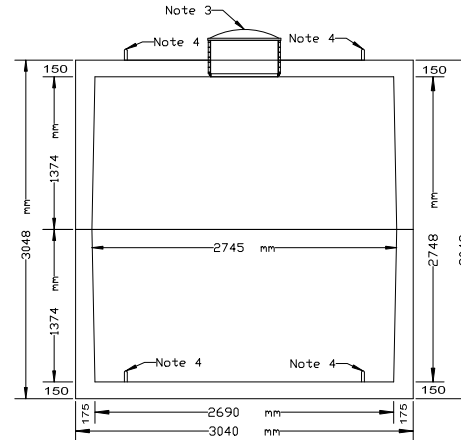
End Elevation Section
