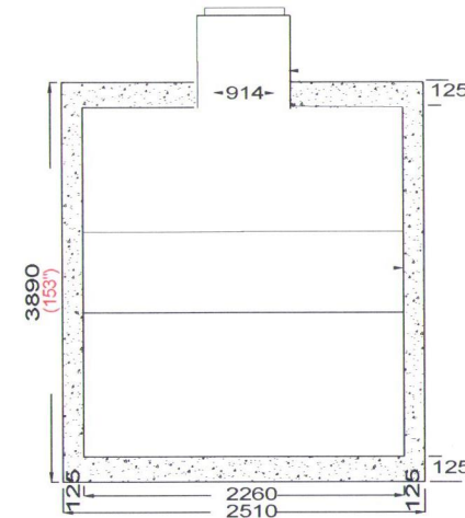
3890 (153") 2260 (89") 2510 (99") End Elevation Section
