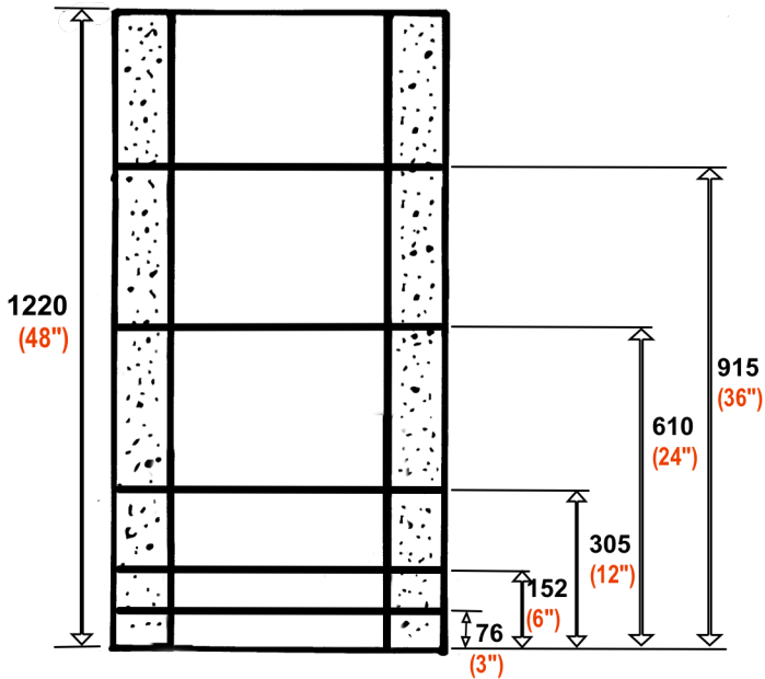
CUTAWAY VIEW Approximate Weight 720 Kg
