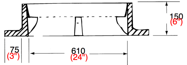
CAST IRON GRATE & FRAME Weight 215 kg. (48Lb)
