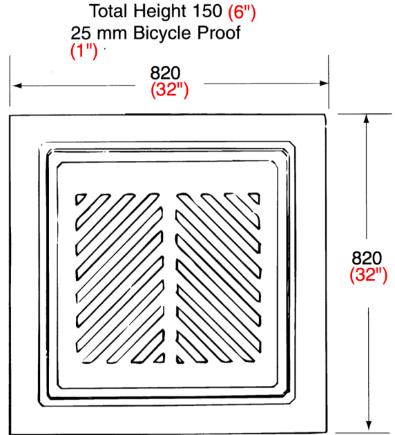
CAST IRON GRATE & FRAME Weight 215 kg. (48Lb)
