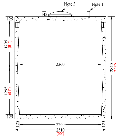
End Elevation Section
