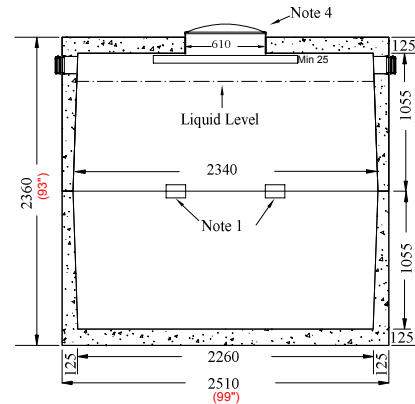
End Elevation Section
