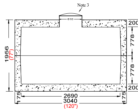
End Elevation Section
