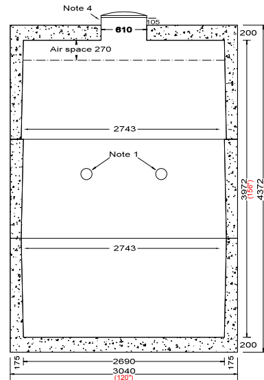
End Elevation Section
