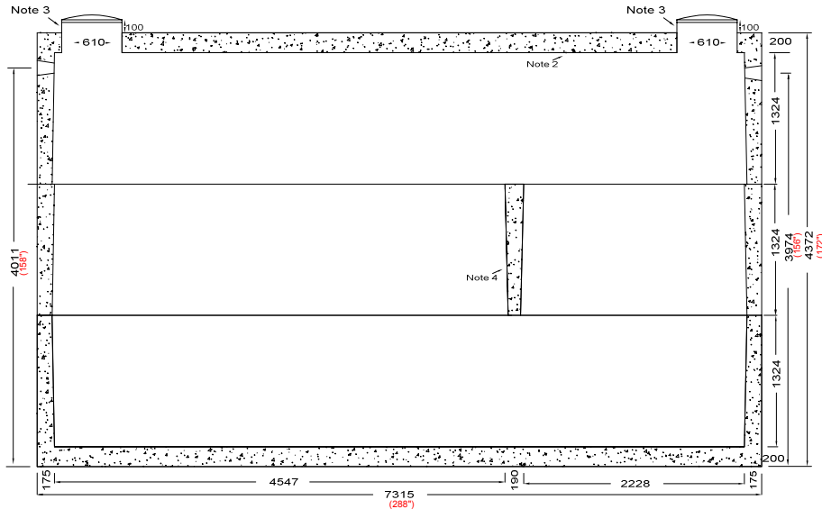
Side Elevation Section
