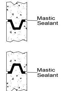
Tongue and Groove Joint
