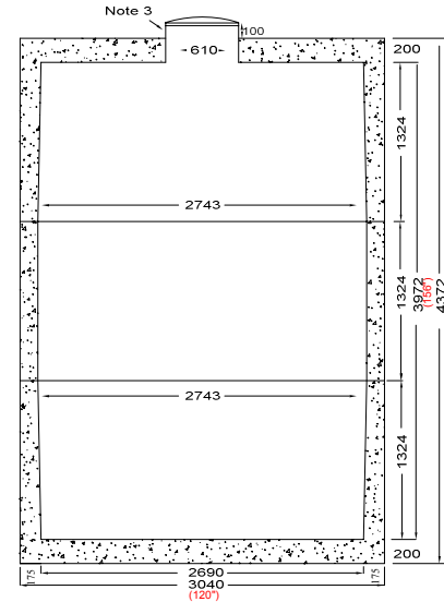
End Elevation Section
