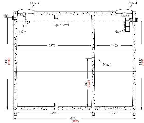
Side Elevation Section
