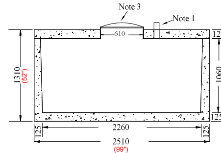
End Elevation Section
