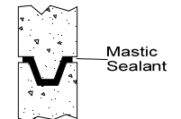
Mastic Sealant
