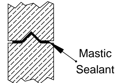
Tongue and Groove Joint
